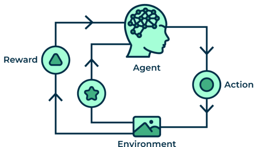
Reinforcement Learning
